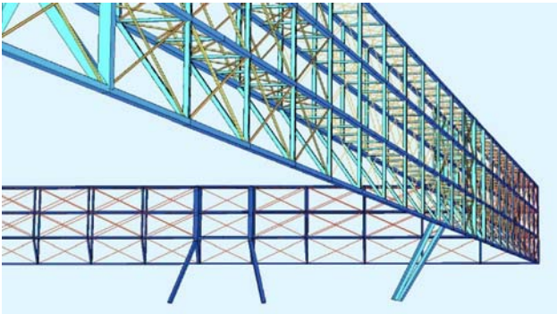
Munich, SWISS-RE Germany, computer model of steel construction
